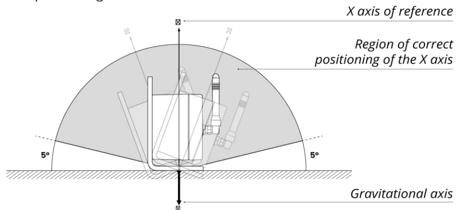
Figure 2 - Tiltmeter side view Display of the “Region of correct positioning”.
